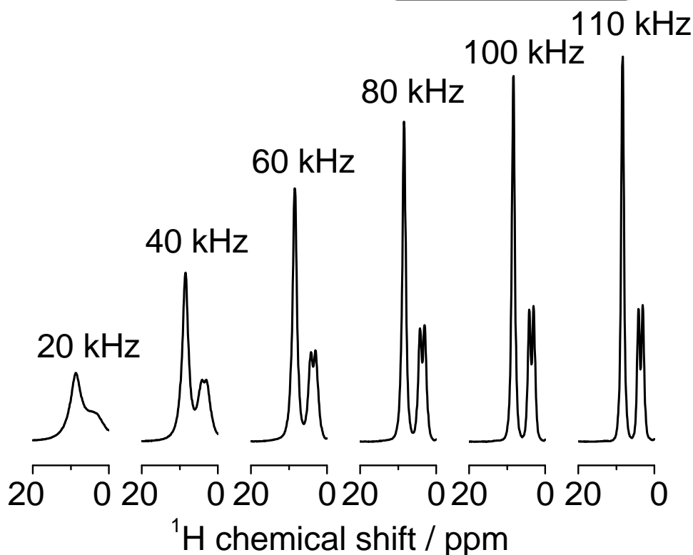
^1\text{H} NMR spectra of glycine at 600 MHz (14.1 T).
