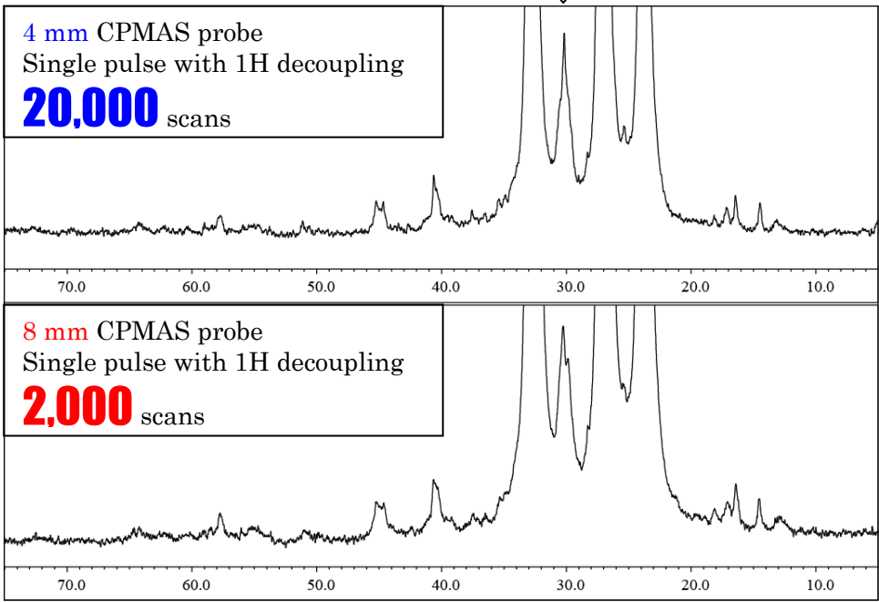
Cross-linked natural rubber with carbon-black Sample courtesy of Prof. Seiichi Kawahara (Nagaoka University of Technology)
